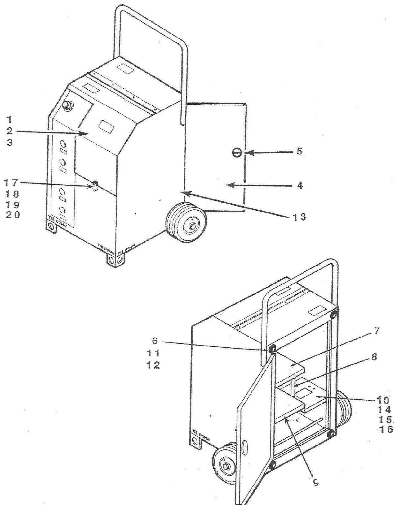
FIGURE 2. FRAME/CABINET ASSEMBLY
