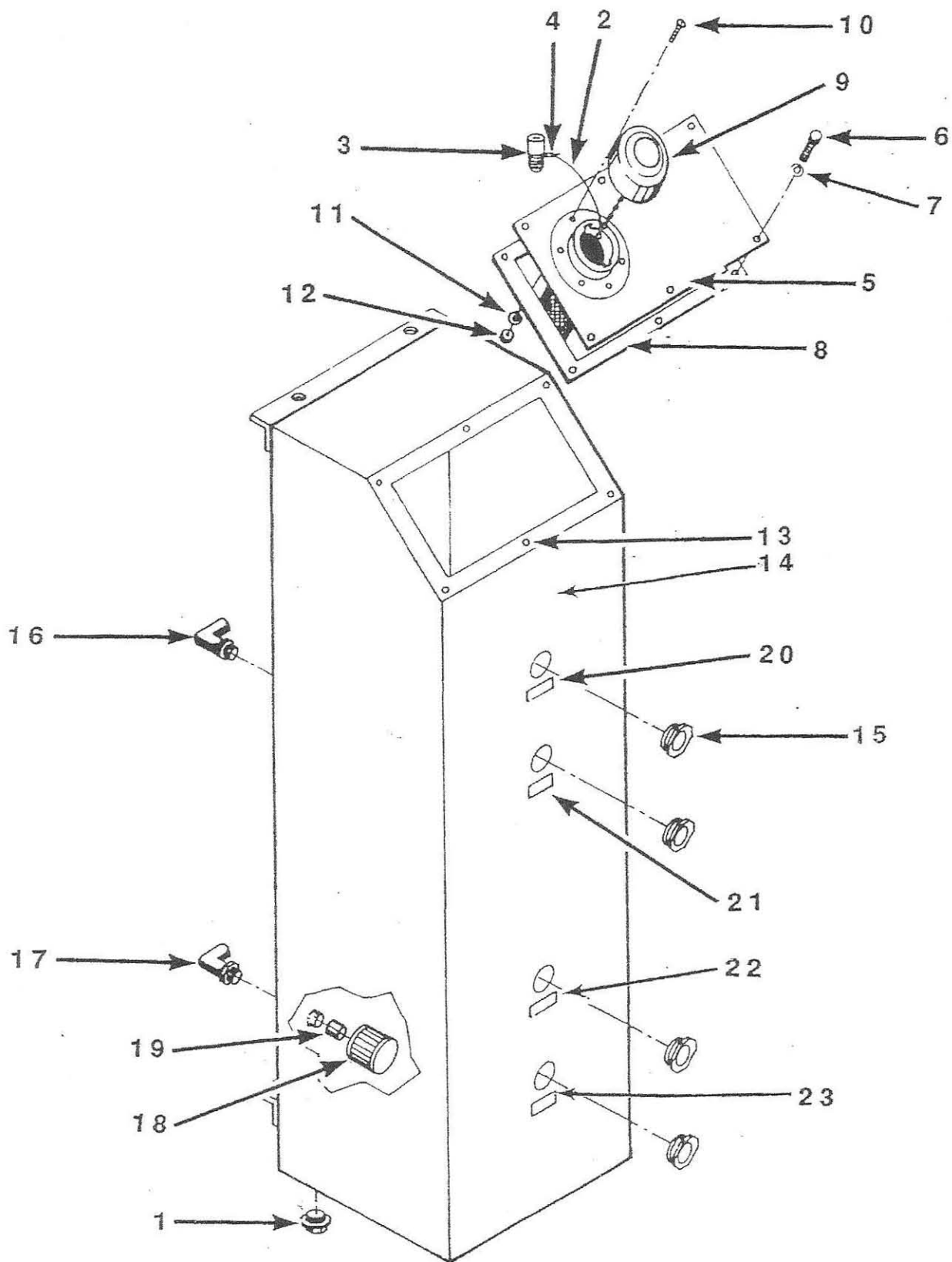
FIGURE 5. RESERVOIR ASSEMBLY
