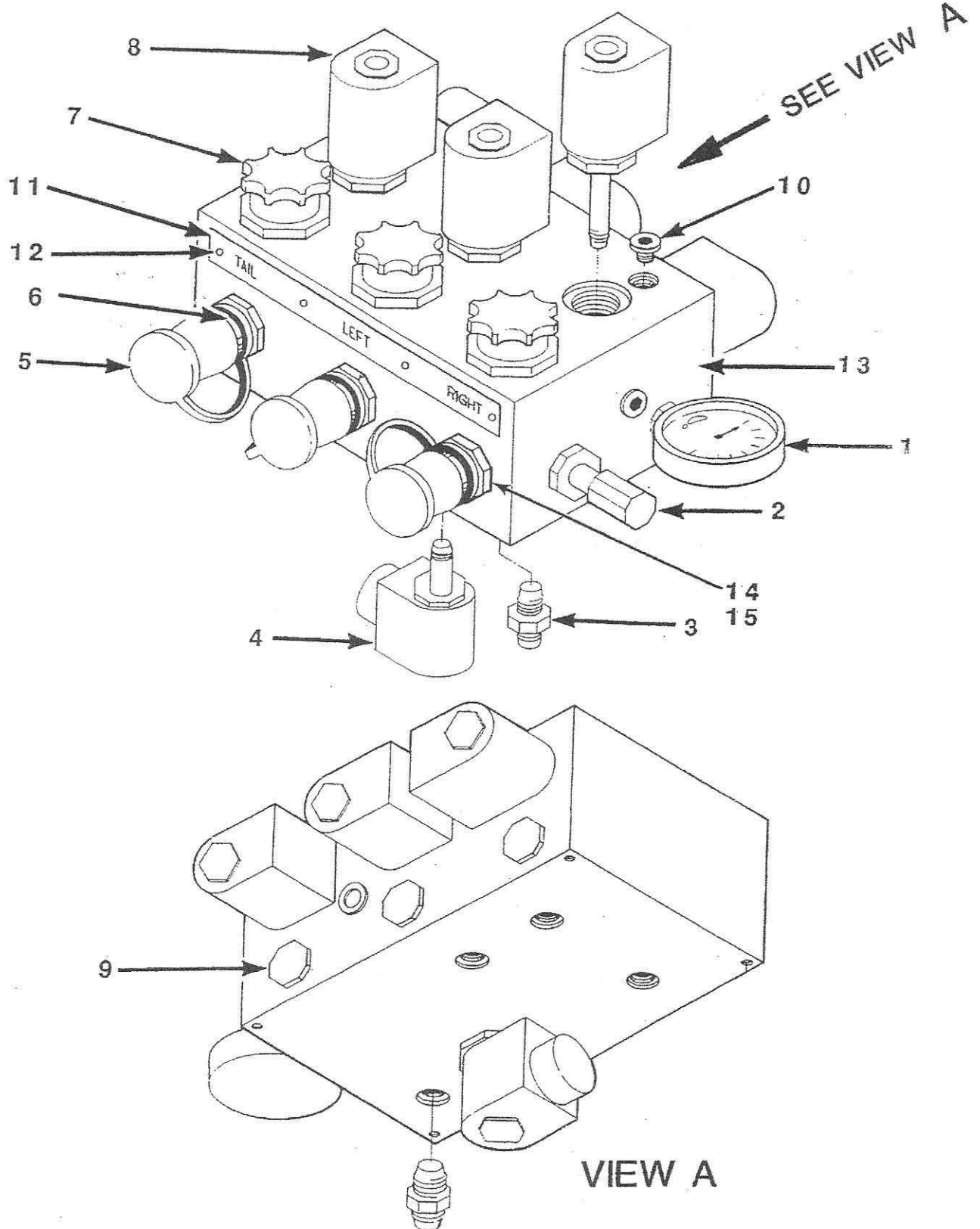
FIGURE 3. MANIFOLD ASSEMBLY
